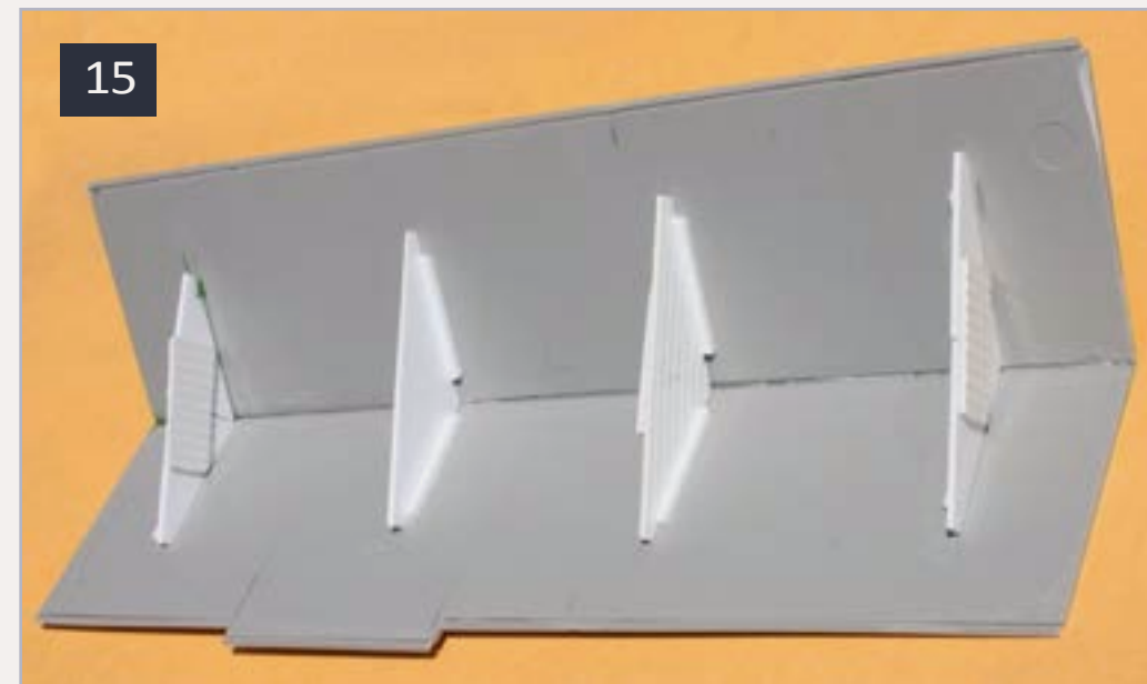
15: When the roof pieces and internal formers are assembled, adding short pieces of scale 6 x 6-inch styrene in the corners, a strong one-piece roof structure is created. The 6 x 6-inch styrene corner pieces are not visible for two of the formers, because they are on the opposite side in this view.
