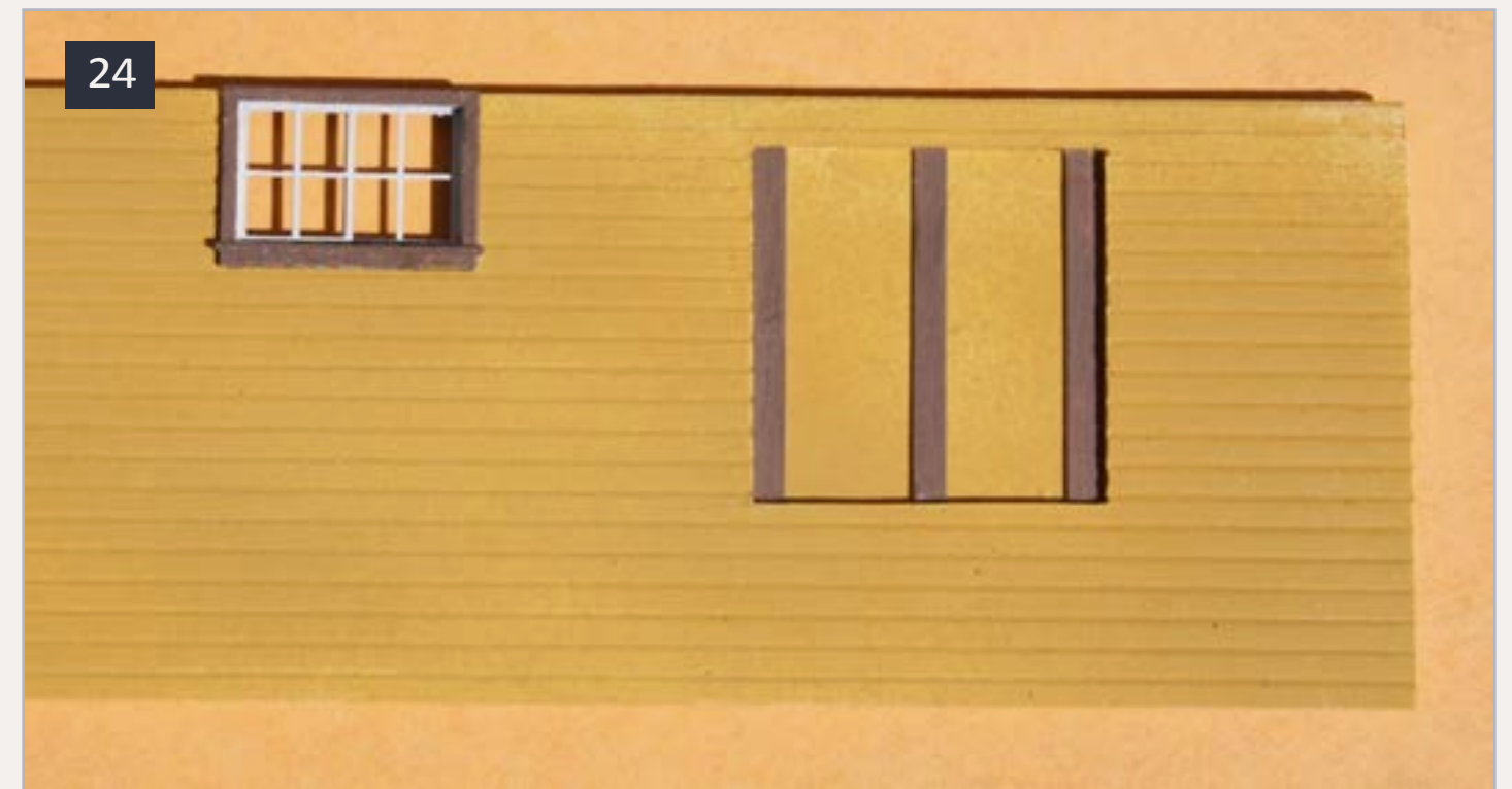
24: The first step in creating the freight doors was to add vertical strips of scale 1 x 8-inch styrene. These had been pre-painted brown. This is the back wall of the depot.
