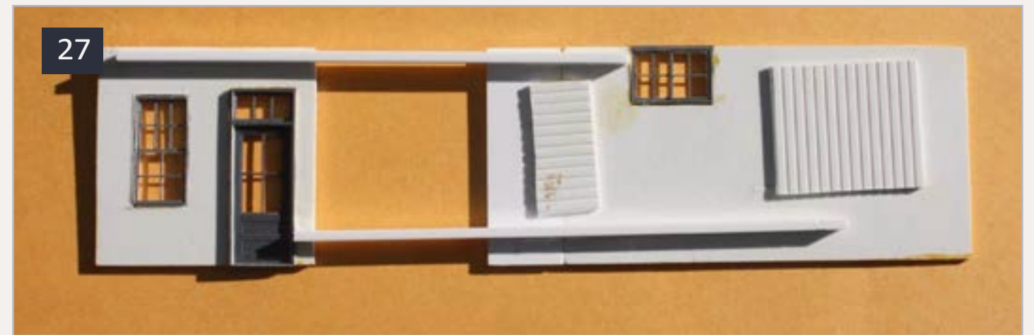
27: Strengthening and aligning the front wall of the depot takes a little extra construction, since this wall has three parts. The two outer parts were connected with styrene strip, as evident in this view of the back of the wall at this point.
