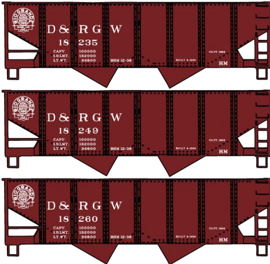
#25804 Denver & Rio Grande Western USRA Hopper 3-Car Set $46.98 Retail
