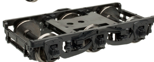
Item #91990001 - HO Scale Passenger Car Trucks 2411
