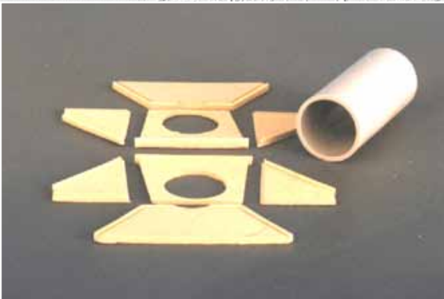
21452 Durchlass - Bausatz, 78x78x48 mm 21452 Concrete pipe culvert, building kit, 78x78x48 mm
