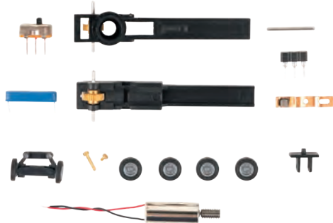
163710 Car System Chassis kit »N-Bus, N-Lorry« Make the stationary vehicle model of your choice fit for Car System. Chassis kit to motorize stationary models of N buses and N trucks for Car System operation. Set contains all vehicle components required for the assembly of a fully functioning two- or three-axle Car System N gauge chassis (bus and truck), except the rechargeable batteries.
