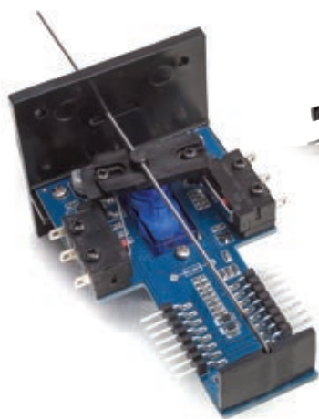
Walthers Controls HO, N, Z, S & O Scales Switch Machine – 942-101
